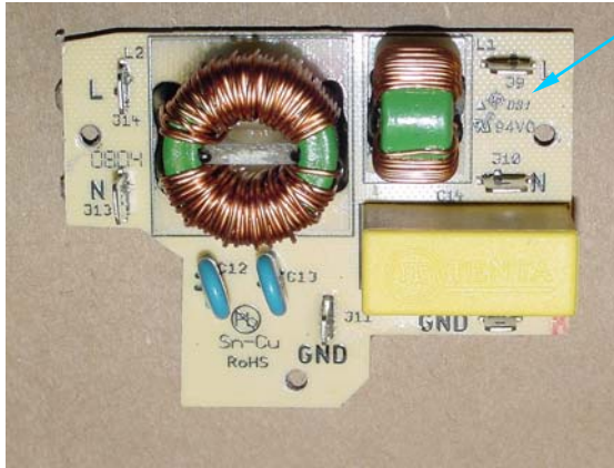
RFI Board 990078800
