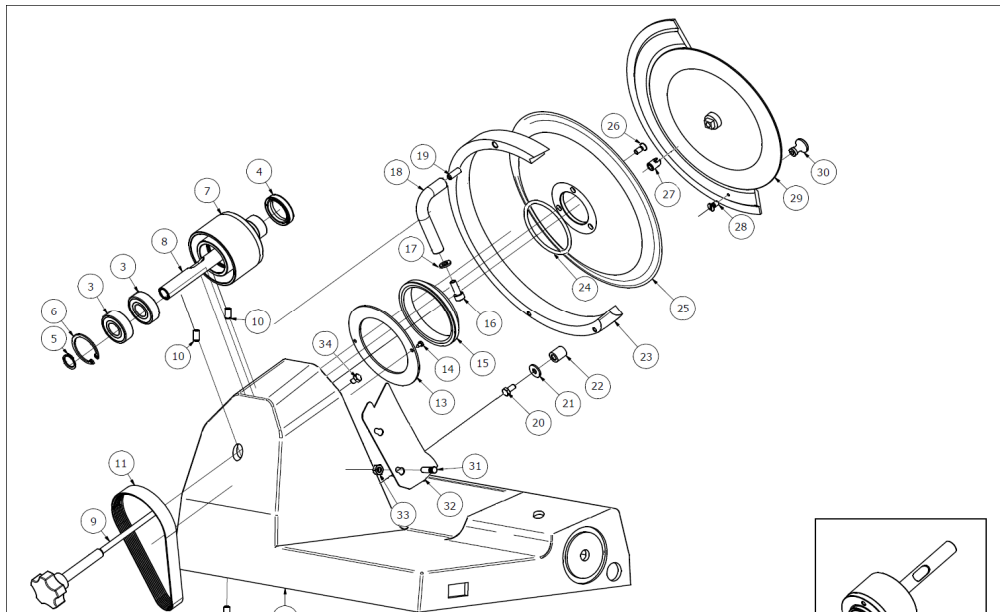
BASE – TRASMISSION – BLADE - TAB.1
