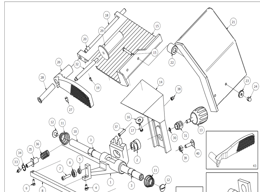
MEAT TABLE ASSEMBLY - TAB.2
