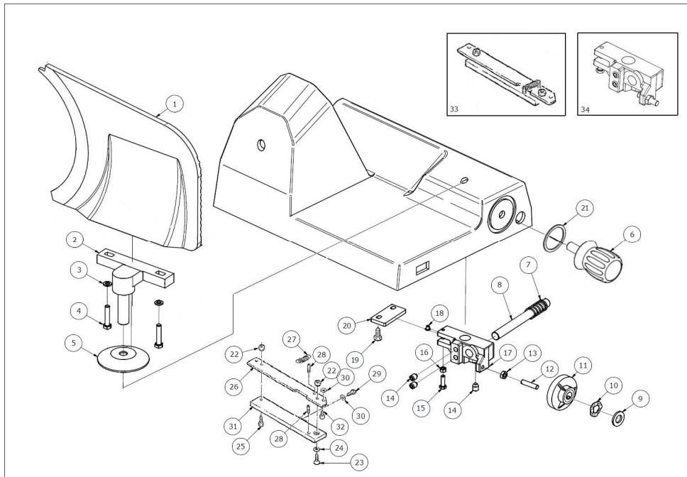
THICKNESS ADJUSTING ASSEMBLY - TAB.3
