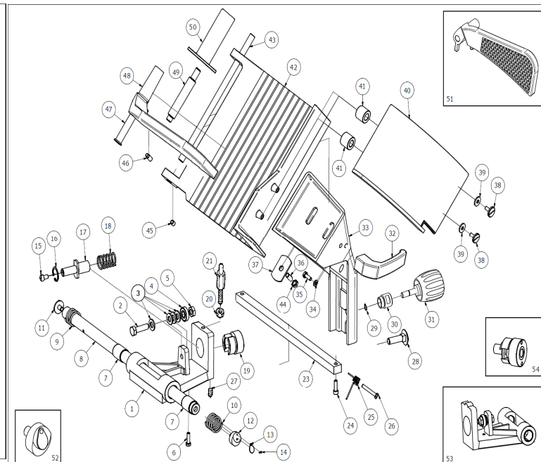
MEAT TABLE ASSEMBLY TAB.2
