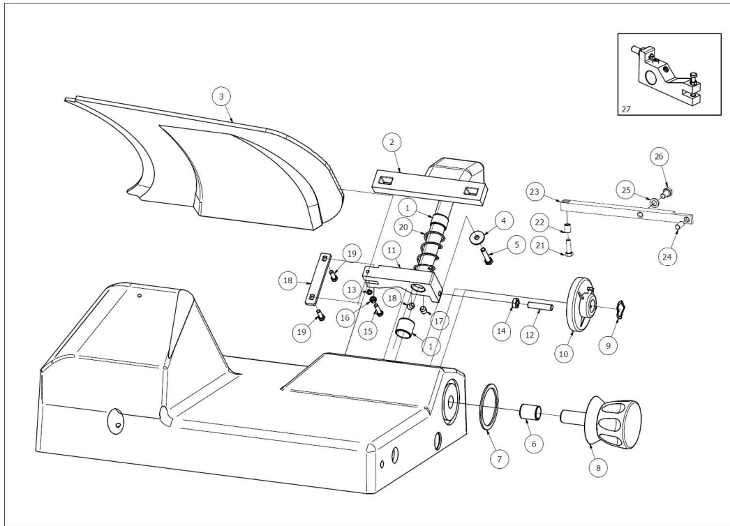
THICKNESS ADJUSTING ASSEMBLY TAB.3
