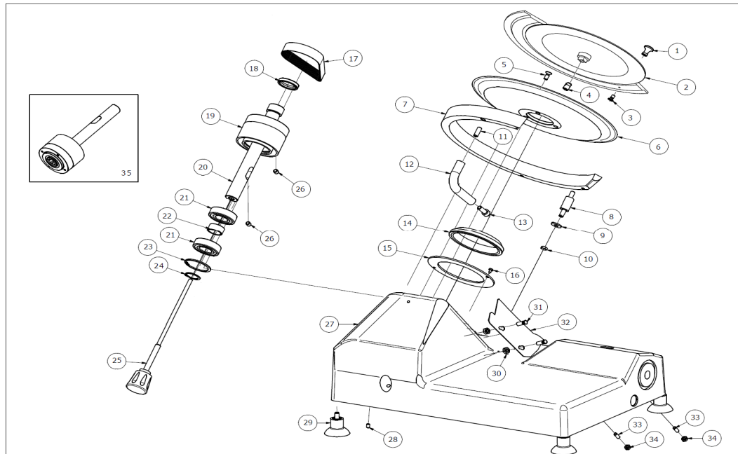
BASE – TRASMISSION – BLADE TAB.1
